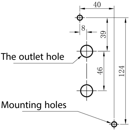
Mounting holes
