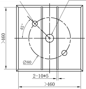
Mounting holes The outlet hole
