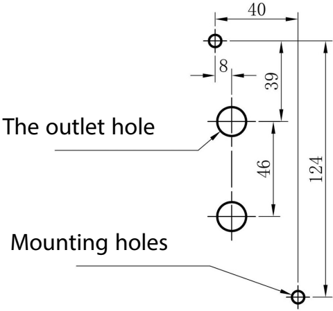
Mounting holes
