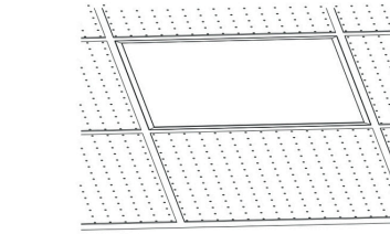
4. Flat the panel, panel frame fixed on ceiling frame
