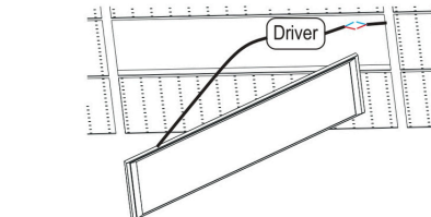
2. Driver connected with home wire
