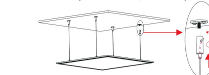
4. Steel wire rope though locker, then locker fixed with flat washer
