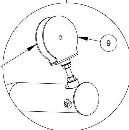
PROPERLY INSTALLED VIEW
