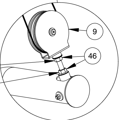
PROPERLY INSTALLED VIEW
