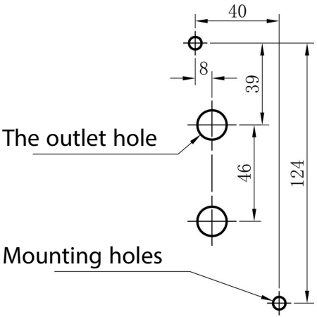
Mounting holes
