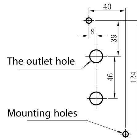
Mounting holes
