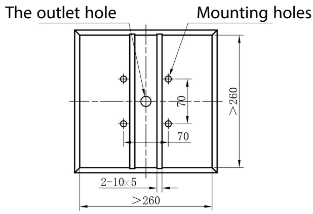
Mounting holes
