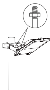
③ Clamp kit for pole installation
