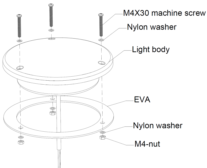
(Installation diagram)
